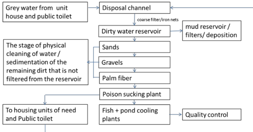
Figure 13. Scheme of grey water treatment horizontal flow
